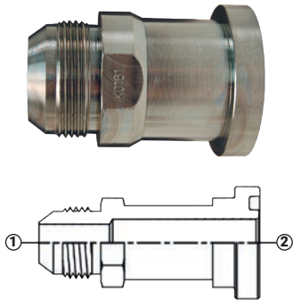
(1) Macho JIC (2) Brida SAE O-Ring
