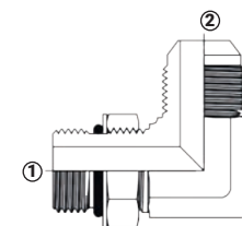
(1) Macho SAE O-ring (2) Macho JIC SAE 070220
