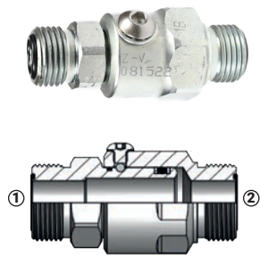
(1) Macho Face Seal (2) Macho Face Seal
